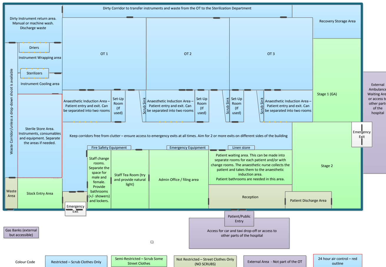
Diagram 5.1: OT Design
