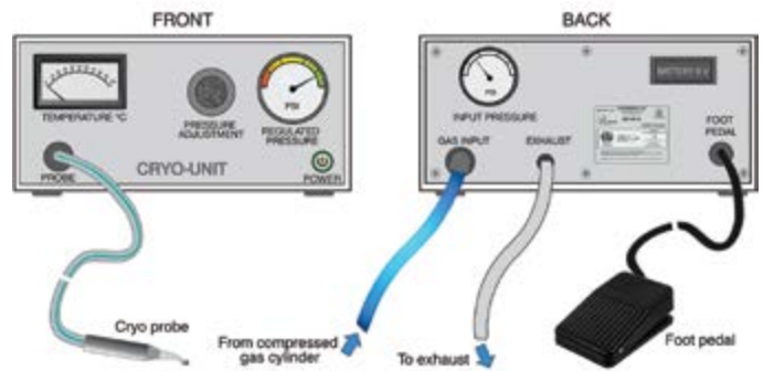
Figure 6.6: Cryotherapy machine
